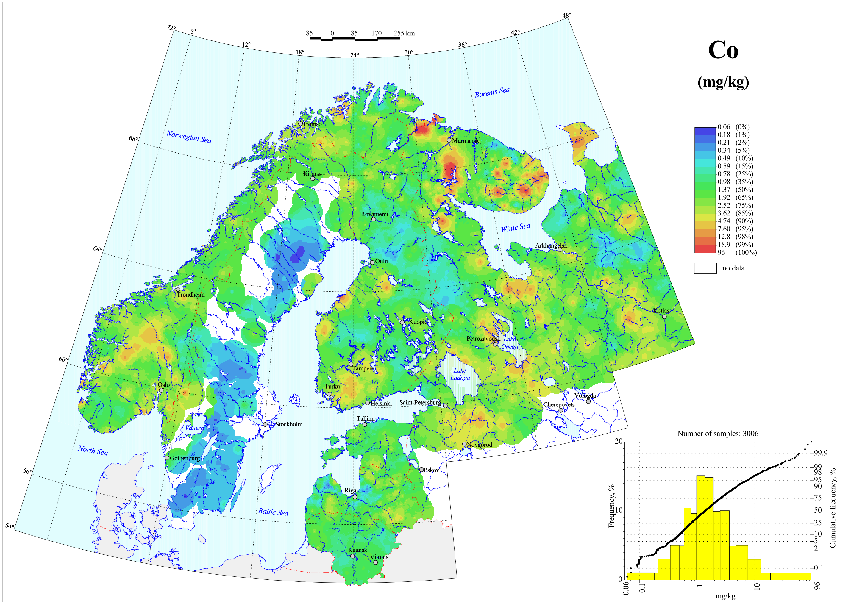
Cobalt in Organic Soil Layer, Total Content
